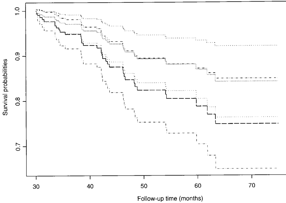
Figure 1. Estimated Conditional Survival Probabilities for the Diabetic Retinopathy Patients. The “—” curve represents the point estimate of the survival function for the adult-onset diabetics; the “.....” curves represent the corresponding 95% confidence limits; the “- - -” curve represents the point estimate of the survival function for the juvenile-onset diabetics; and the “- . - . -” curves represent the corresponding 95% confidence limits.
